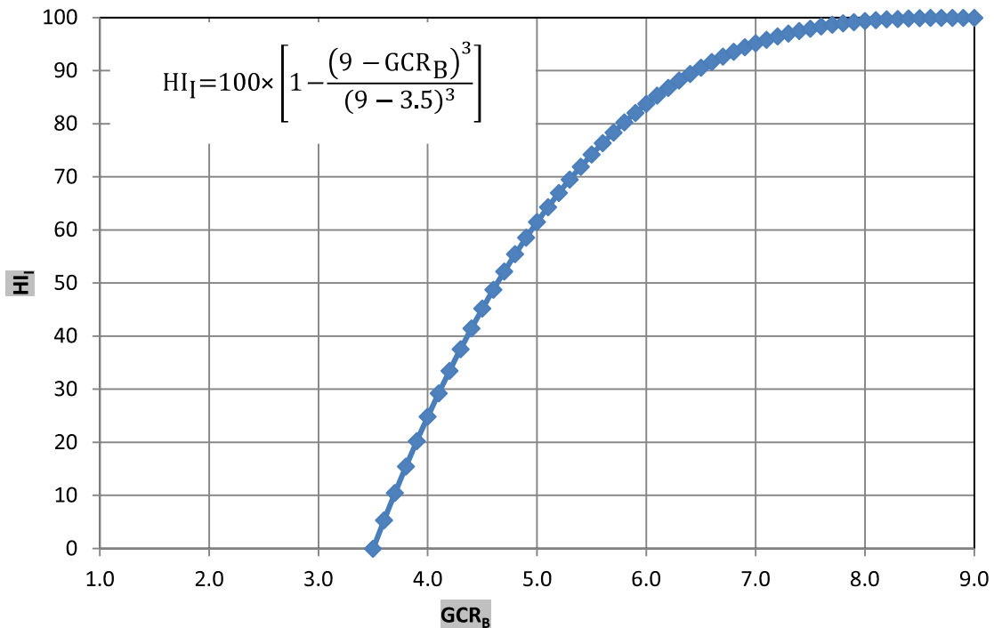
Figure 7 - Blended General Condition Rating vs. Interim Health Index
